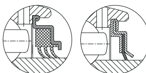
R3 SEAL
